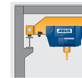
Standard main girder connection configuration Version 3
