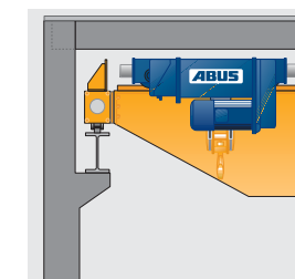
Stooled down configuration Version 1
