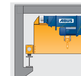
Standard main girder connection configuration Version 3
