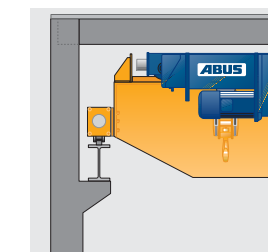
Stooled down configuration Version 2
