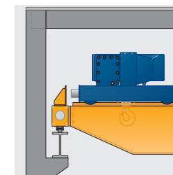
Standard main girder connection configuration - Version 1
