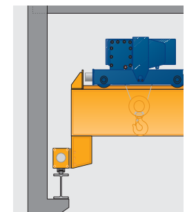
Stooped up configuration Version 5
