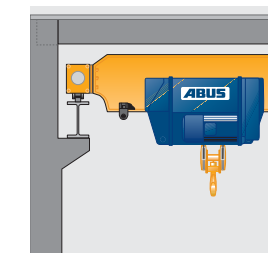
Stooled down configuration Version 2
