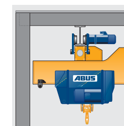
Standard main girder connection configuration Version 1, "angled" (variable overhang for minimum side approach dimension)
