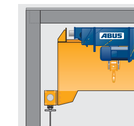
Stooled up configuration Version 4
