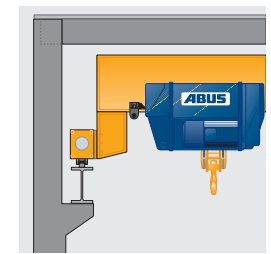
Stooled up configuration Version 5
