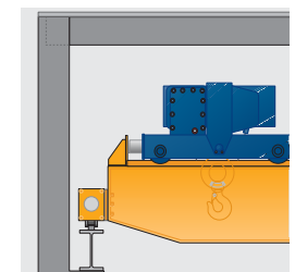
Stooped up configuration Version 2
